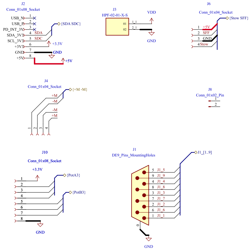
Main Board Connectors
