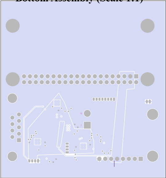
Bottom Assembly (Scale 1:1)
