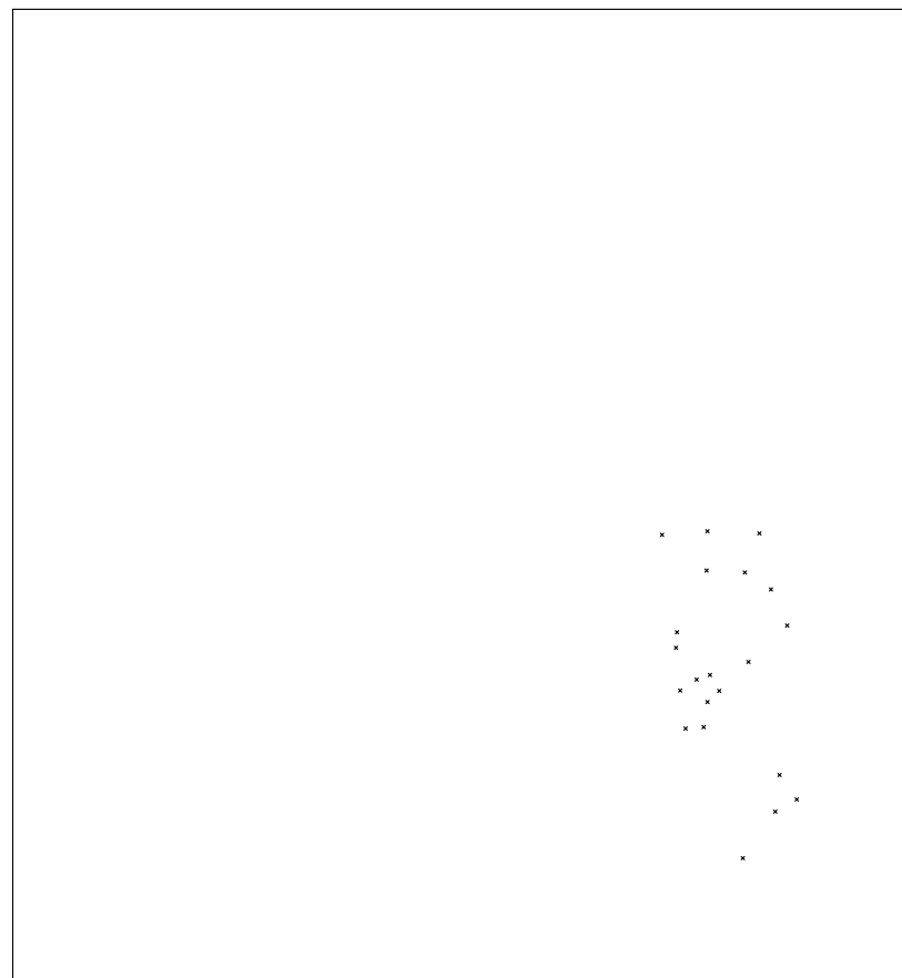
Drill Map: x 0.250mm / 0.0098" (21 holes)
