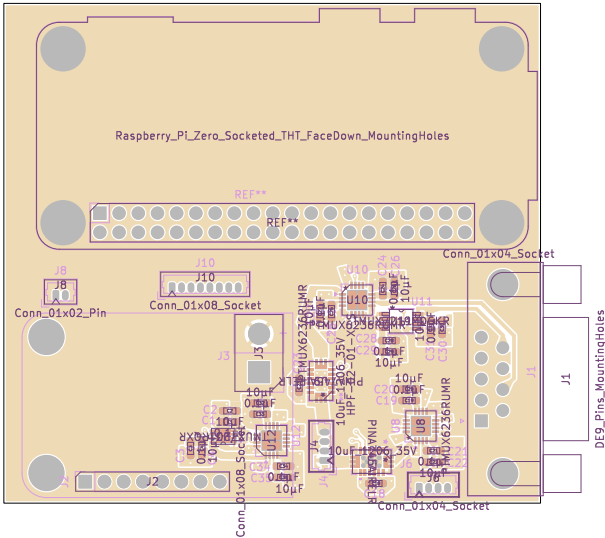
Top Assembly (Scale 1:1)
