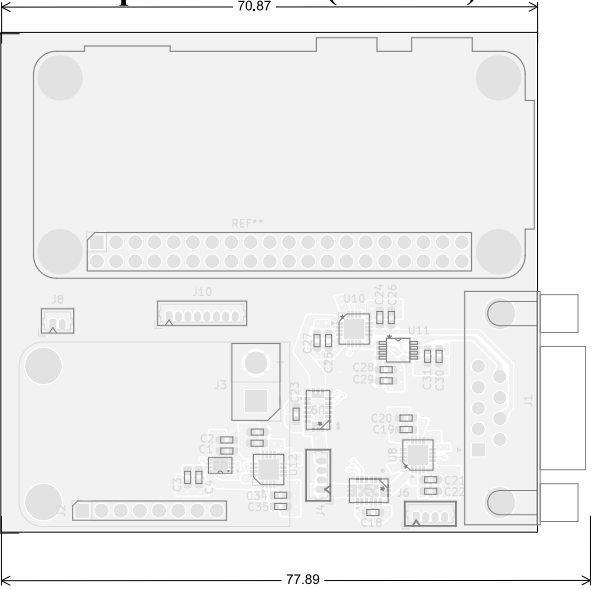
Top Fabrication (Scale 1:1)
