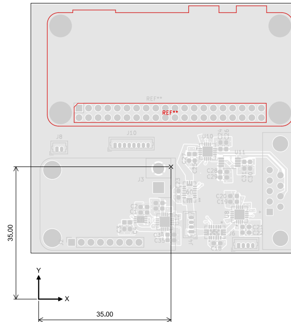
Top Test Points (Scale 1:1)
