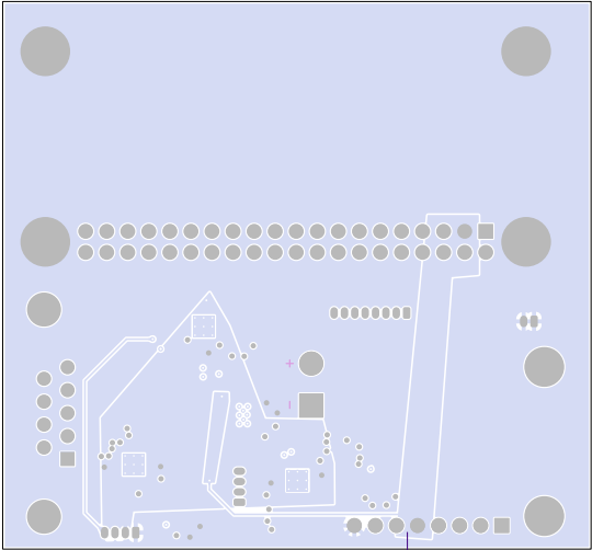
Bottom Assembly (Scale 1:1)
