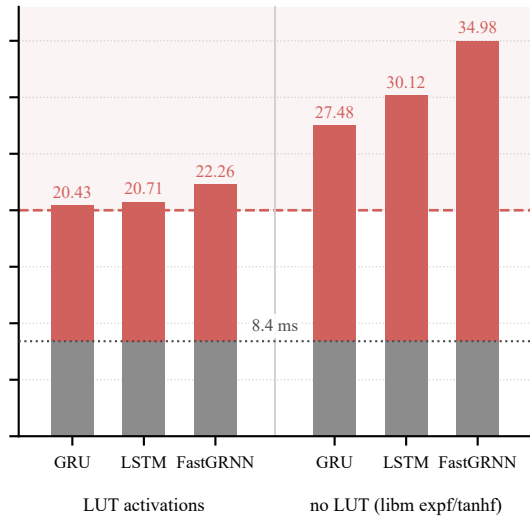
(b) I^2C @ 10 \text{ kHz}
