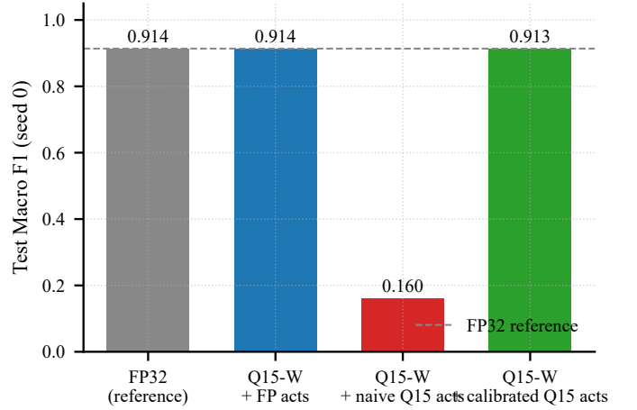
Fig. 5. Quantization modes on seed-0 model. Weight-only Q15 is lossless; naive Q15 activations collapse the model; calibrated Q15 activations recover the reference within rounding noise.
