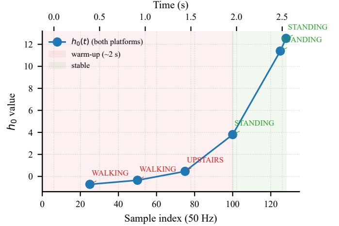
Fig. 8. Hidden-state component h_0 and emitted class label over a single 2.56 s window (50 Hz, STANDING ground truth). Both Arduino and MSP430 produce identical trajectories. The class label is unstable until \sim 2 s of history accumulates.
