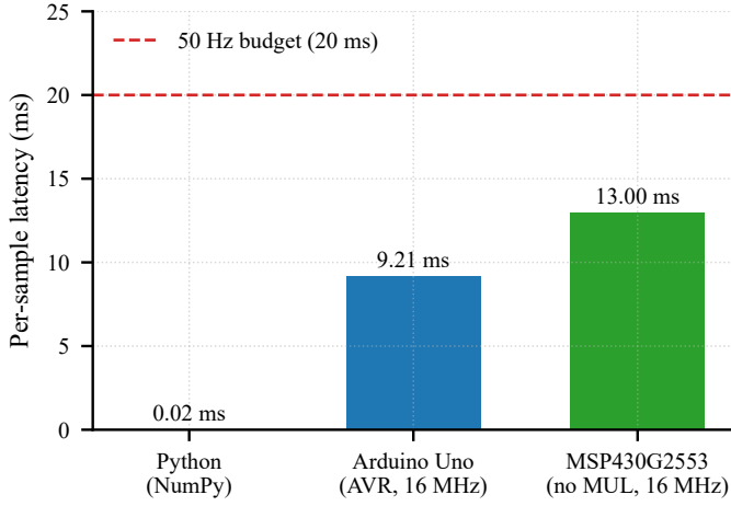
Fig. 7. Per-sample inference latency on the three reference platforms. The red dashed line marks the 20 ms budget imposed by 50 Hz sampling. Both MCU targets execute well below budget.
