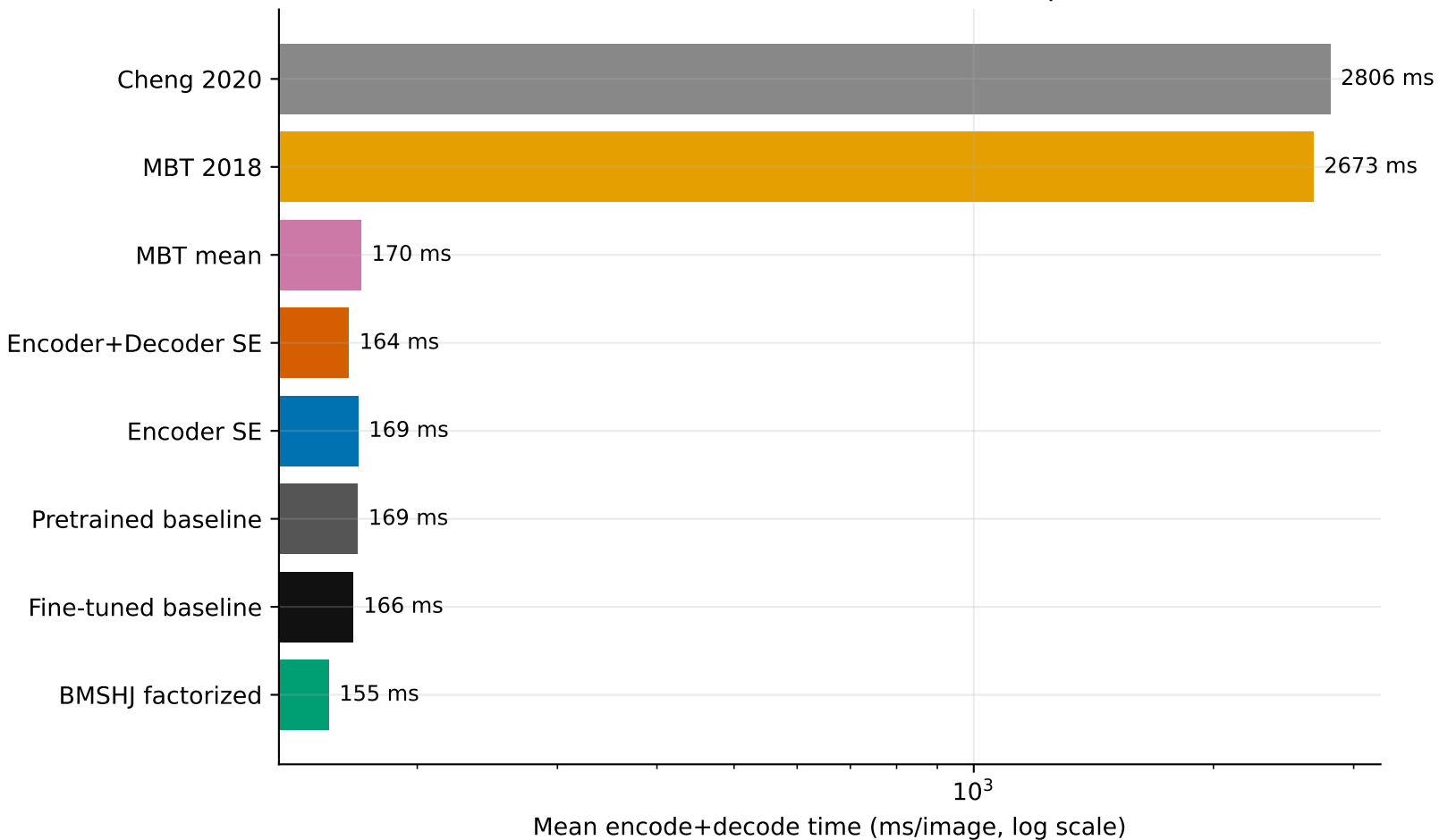
Evaluation runtime across local reference implementations
