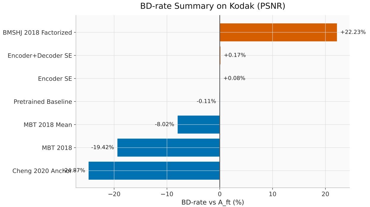
Figure 10: PSNR BD-rate against the fine-tuned vanilla baseline. This view is easier to read than the full multi-model RD curve and makes the large gap between the SE variants and stronger reference priors immediately visible.
