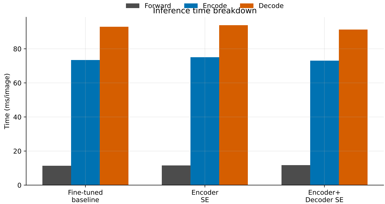
Figure 11: Evaluation-time breakdown for the three main project variants. The forward pass is small compared with entropy coding, and the SE variants stay close to the fine-tuned baseline in all three components.
