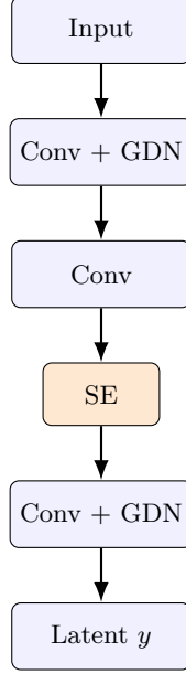
Figure 3: Encoder-side view. In the attention variants, one SE block is inserted between the middle encoder stages.
