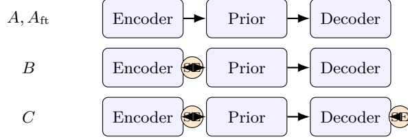
Figure 6: Variant comparison. The project modifies only the transform network: B adds encoder attention, and C adds both encoder and decoder attention.
