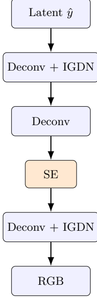
Figure 5: Decoder-side view. Only variant C adds the highlighted decoder SE block.
