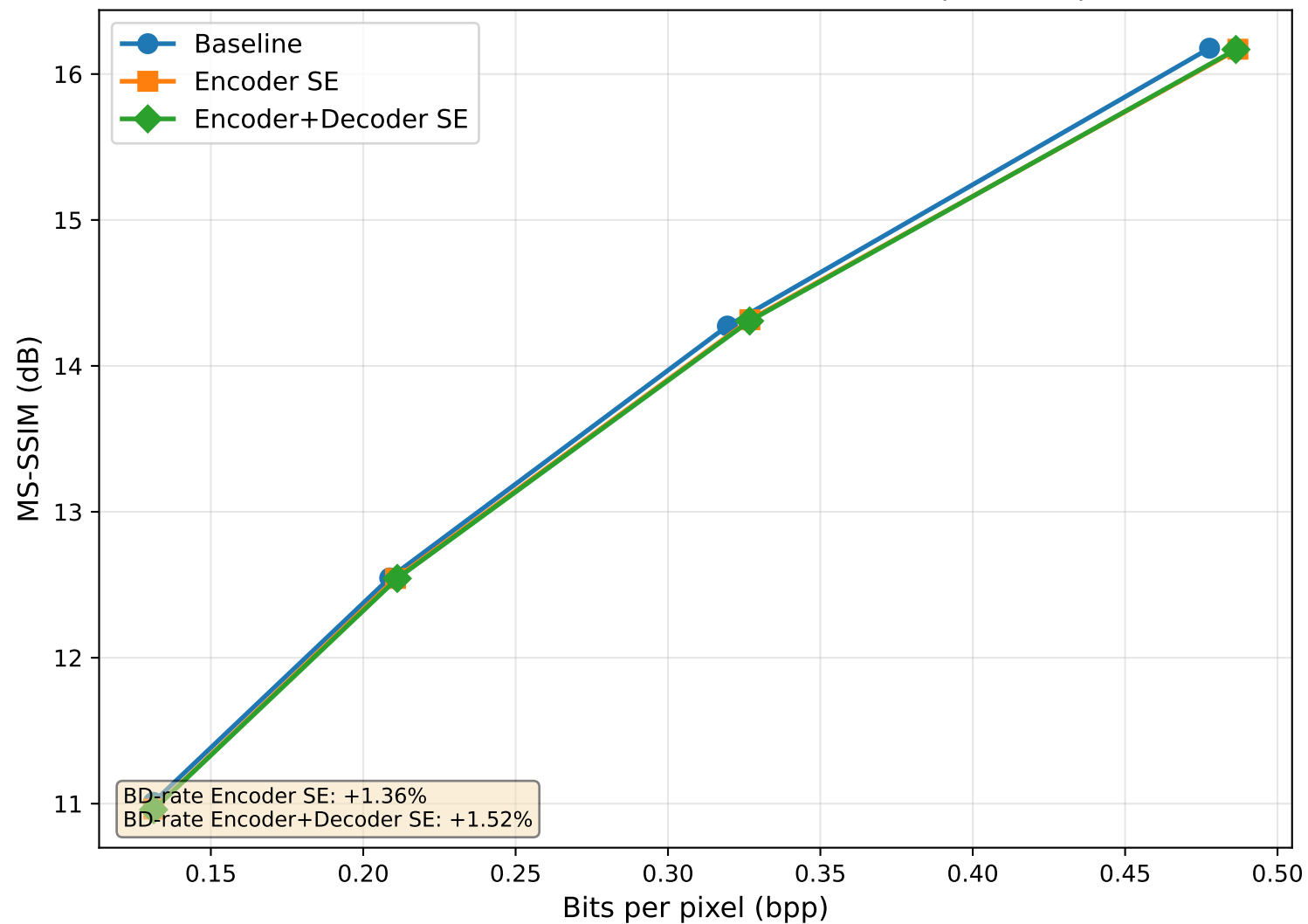
Rate-Distortion Performance on Kodak (MSSSIM)
