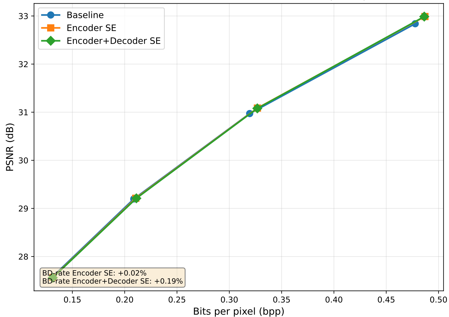
Rate-Distortion Performance on Kodak (PSNR)
