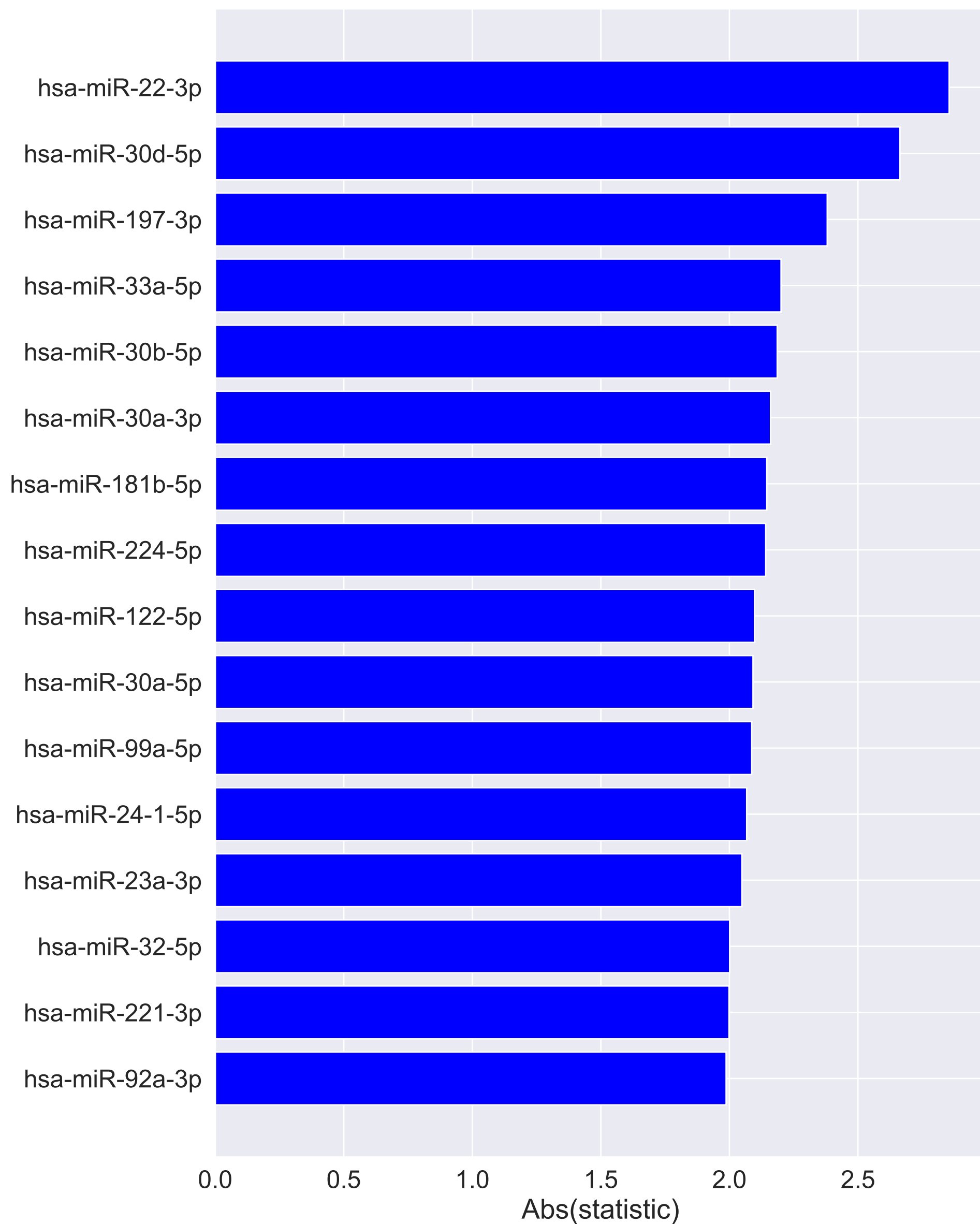
t-Test Feature Importance of Top Differentiating microRNAs
