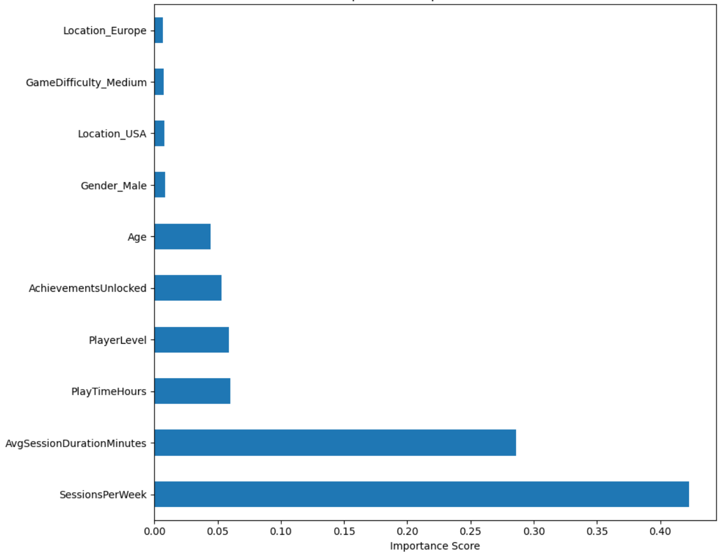
Top 10 Most Important Features
