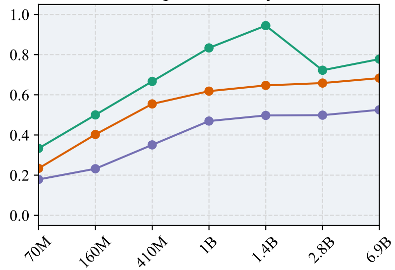
Top-5 Accuracy
