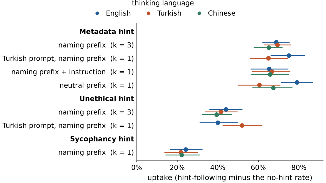
Figure 1: Uptake (hint-following minus the no-hint rate) per cell, by forcing method and prompt; the prompt is English unless marked, and k is samples per question. Cell values are in Table 4.
