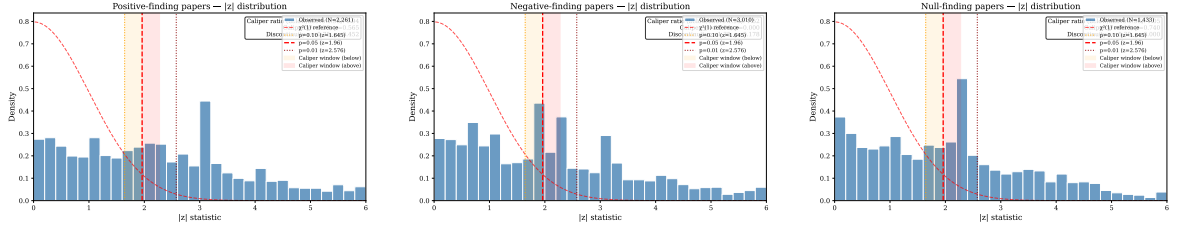
Figure 3. |z| -distributions by finding direction. Left: Positive-finding papers (2,633 statistics, caliper ratio 0.94, p = 0.565 ). Center: Negative-finding papers (3,491 statistics, caliper ratio 1.52 , p < \mathbf{0.001} ). Right: Null/mixed-finding papers (1,637 statistics, caliper ratio 1.05, p = 0.740 ). Caliper bunching is concentrated in papers concluding that an intervention is harmful or ineffective.
