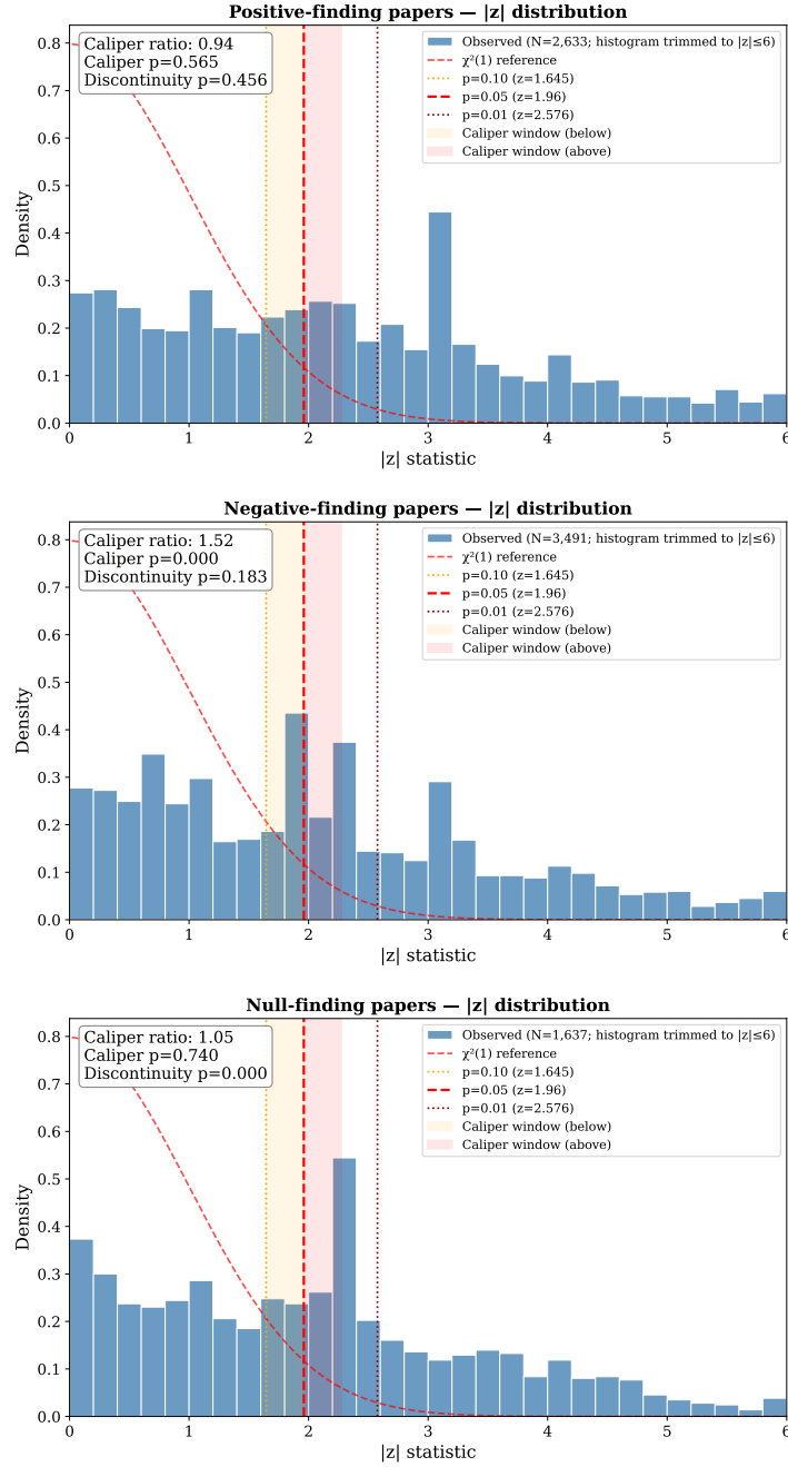
Figure 4. Test-statistic distributions broken out by the paper’s main conclusion. All p -values in this caption are caliper-test p -values; the density discontinuity test gives a different reading for the null/mixed panel and we note it explicitly. Top: Papers finding that a government intervention was beneficial (2,633 statistics; no caliper-test clustering, caliper p = 0.565 ; discontinuity p = 0.456 , no conflict). Middle: Papers finding that an intervention was harmful or ineffective (3,491 statistics; significant caliper-test clustering on the just-below-1.96 side, caliper p < 0.001 ; discontinuity p = 0.183 ). Bottom: Papers with inconclusive or mixed findings (1,637 statistics; no caliper-test clustering, caliper p = 0.740 ). Note that the discontinuity test for null/mixed papers gives p < 0.001 ; as with the JF density anomaly, we prioritize the caliper ratio for the substantive interpretation (Section 5.1). Under the caliper test, near-threshold clustering is concentrated in negative-finding papers; the discontinuity test also flags the null/mixed panel.
