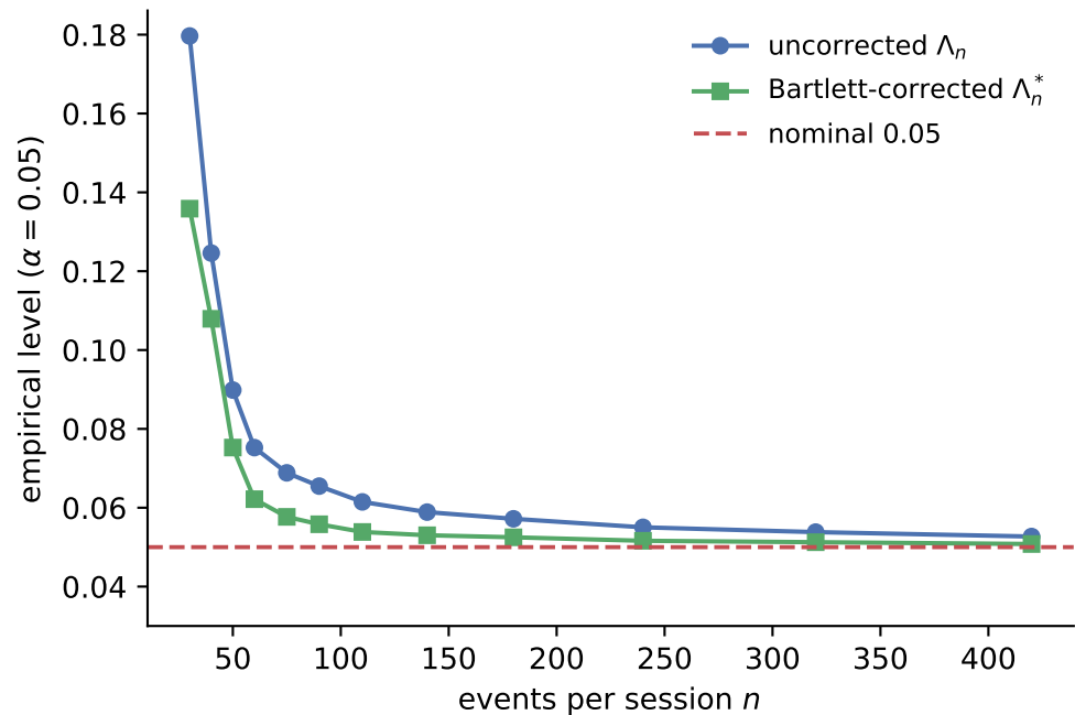
(b) Correction restores calibration
