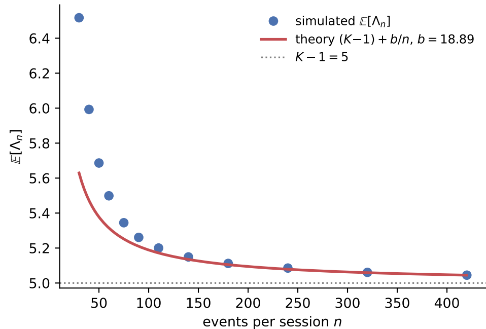
(a) Second-order bias law
