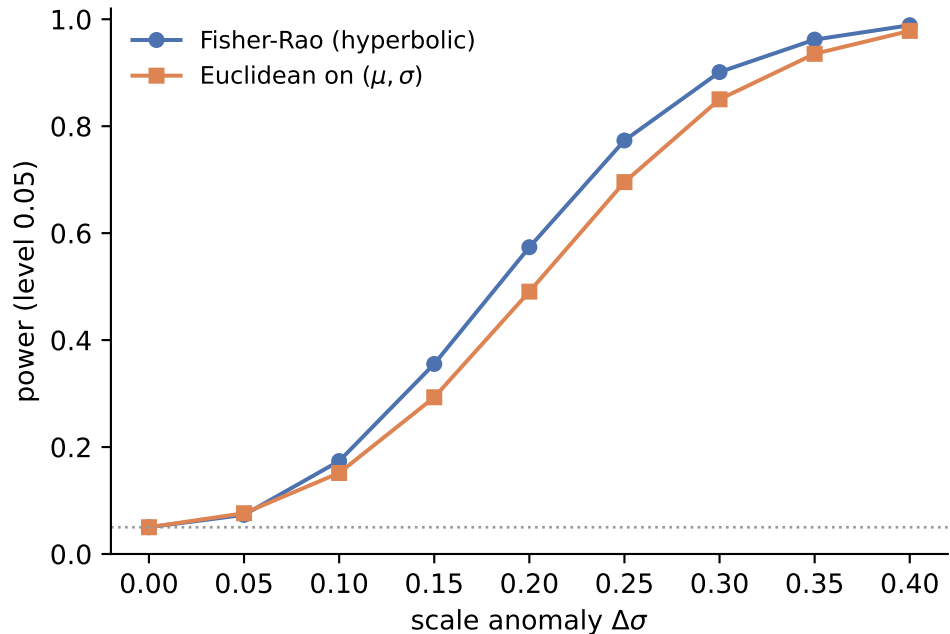
(b) Detecting a scale anomaly
