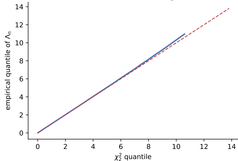
(a) Gaussian manifold: \Lambda_n \rightarrow \chi^2_2 ( n = 200 )
