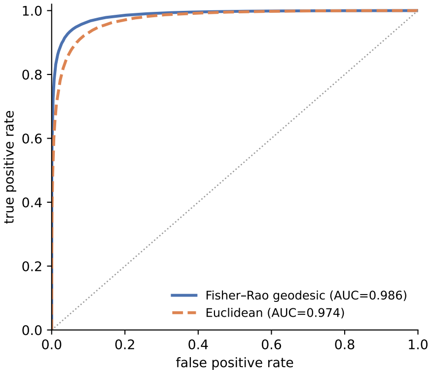
Anomaly detection ROC (severity s=0.5 )
