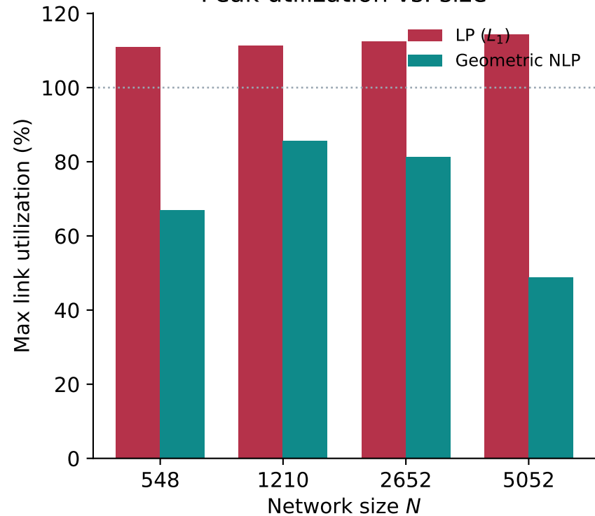
Peak utilization vs. size
