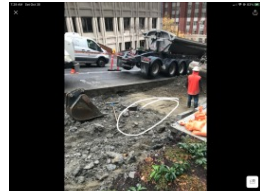
Water line and valve in cased in CDF, PC0014.01 vac truck hydro excavate ITS trench.
