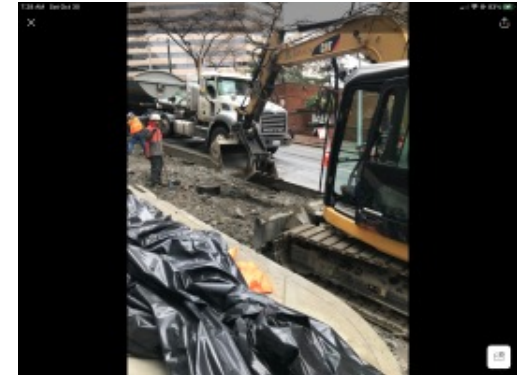
308 Caterpillar excavator cutting sub grade common excavation
