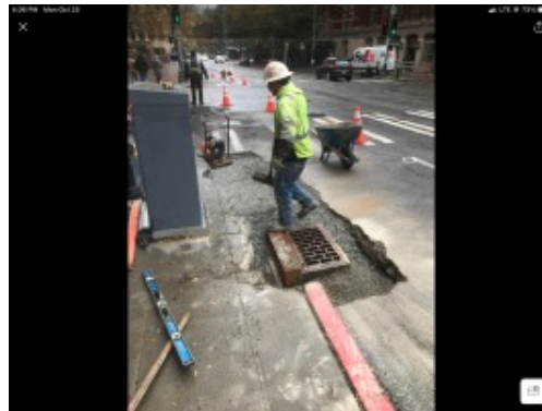
Backfilling and cleaned work area around inlet 1B.
