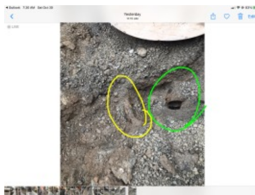
Unlocated gas line in front of 6 inch sewer pipe not connected to clay sewer pipe.
