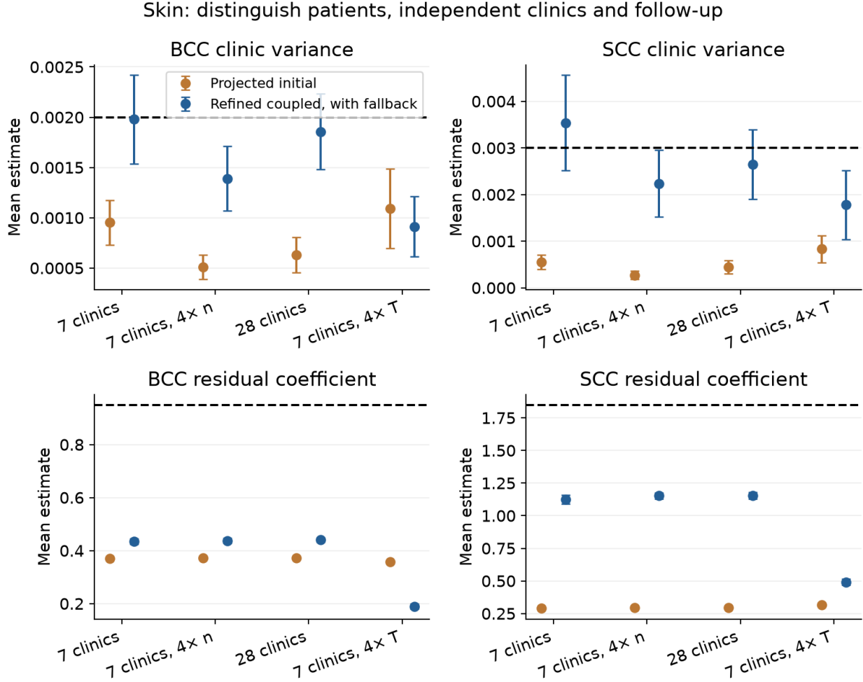
Figure 1. Operational estimates use all certified-initial histories. Error bars on mean estimates are 1.96 Monte Carlo standard errors; dashed lines mark truth. Increasing patients, independent clinics and individual history length are different changes in information.
