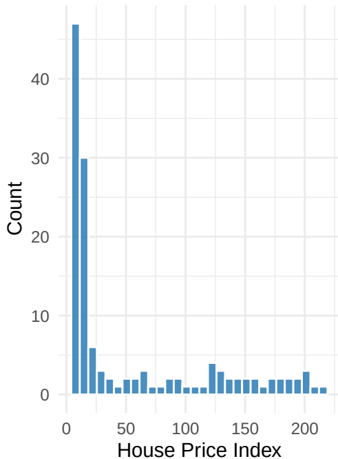
HPI Distribution
