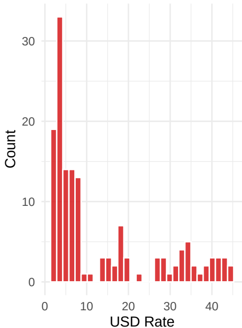
USD/TRY Distribution
