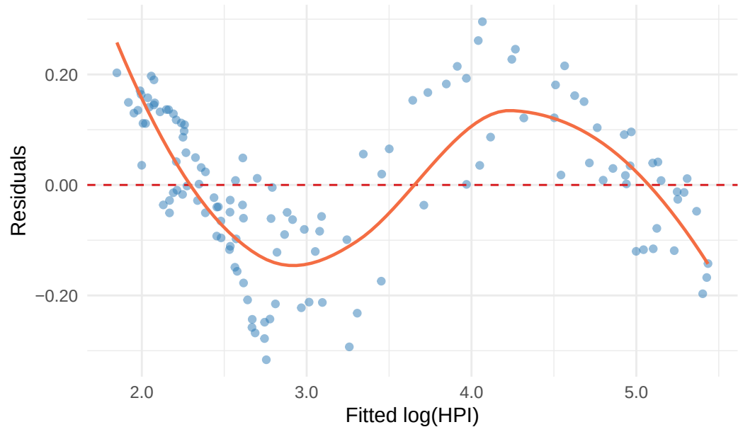
Figure 11. Residuals vs. Fitted Values
