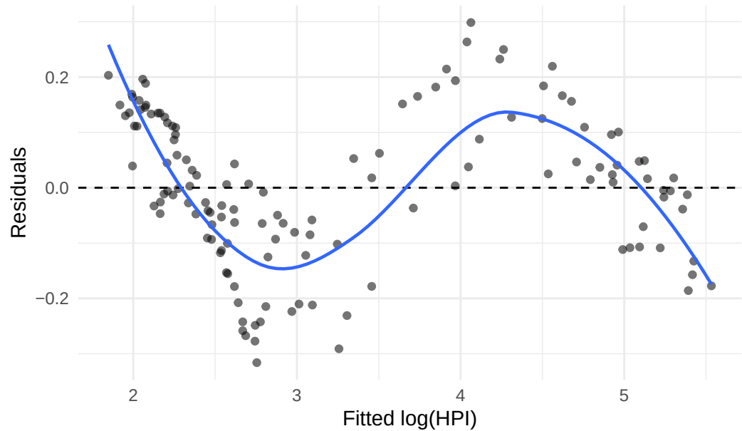
Figure 12. Residuals vs. Fitted Values
