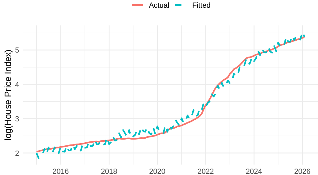
Figure 11. Actual vs. Fitted \log(\text{HPI})
