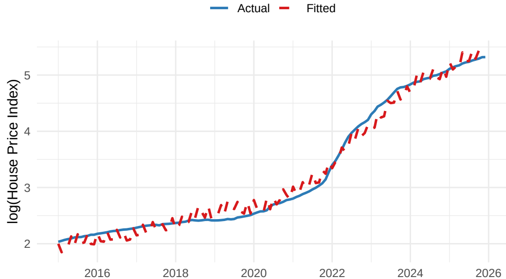
Figure 10. Actual vs. Fitted \log(\text{HPI}) – Full Model
