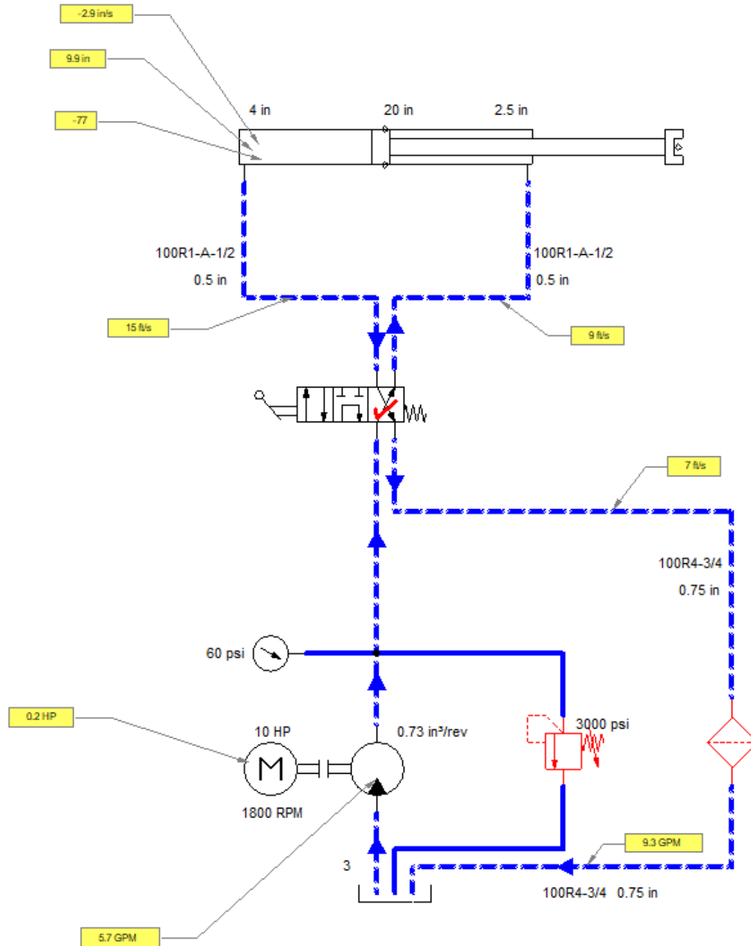
Figure 2- cylinder retracting at full load
