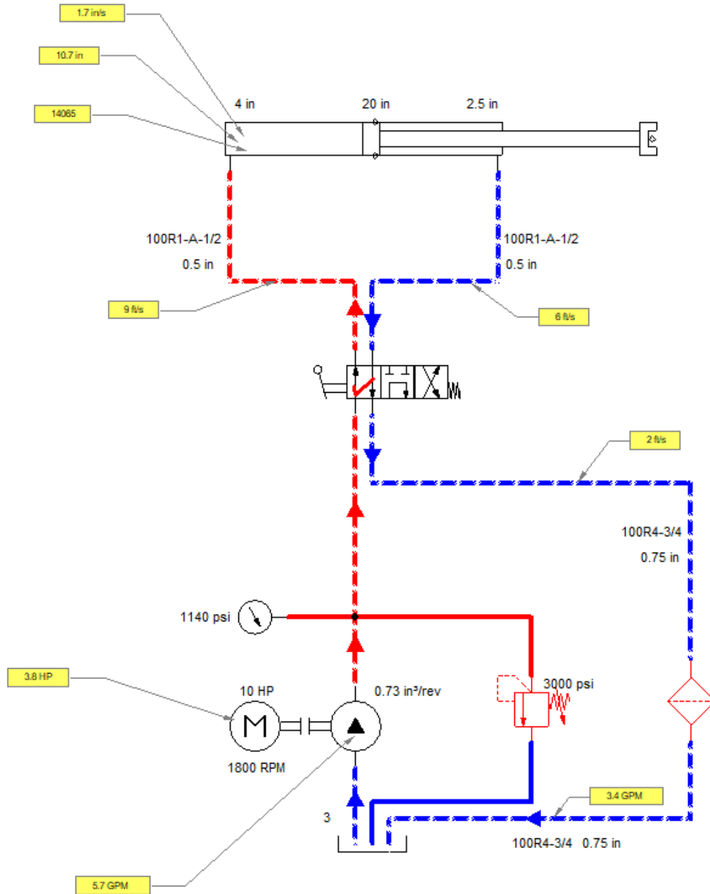
Figure 1- cylinder extending at full load
