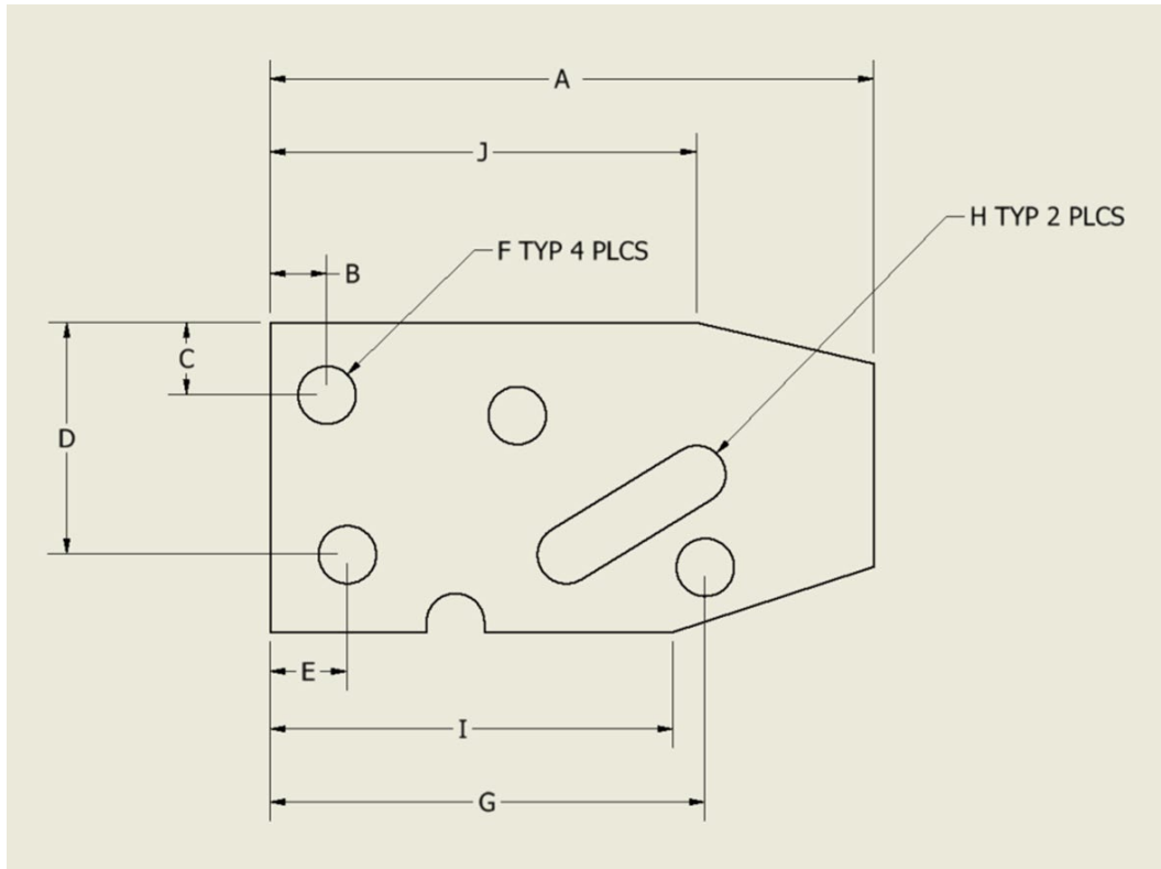
Figure 5 Labeled Part Drawing
