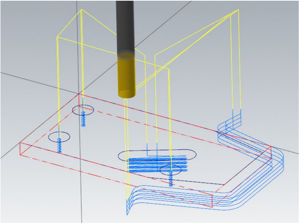
Figure 3 Backplots of all operations
