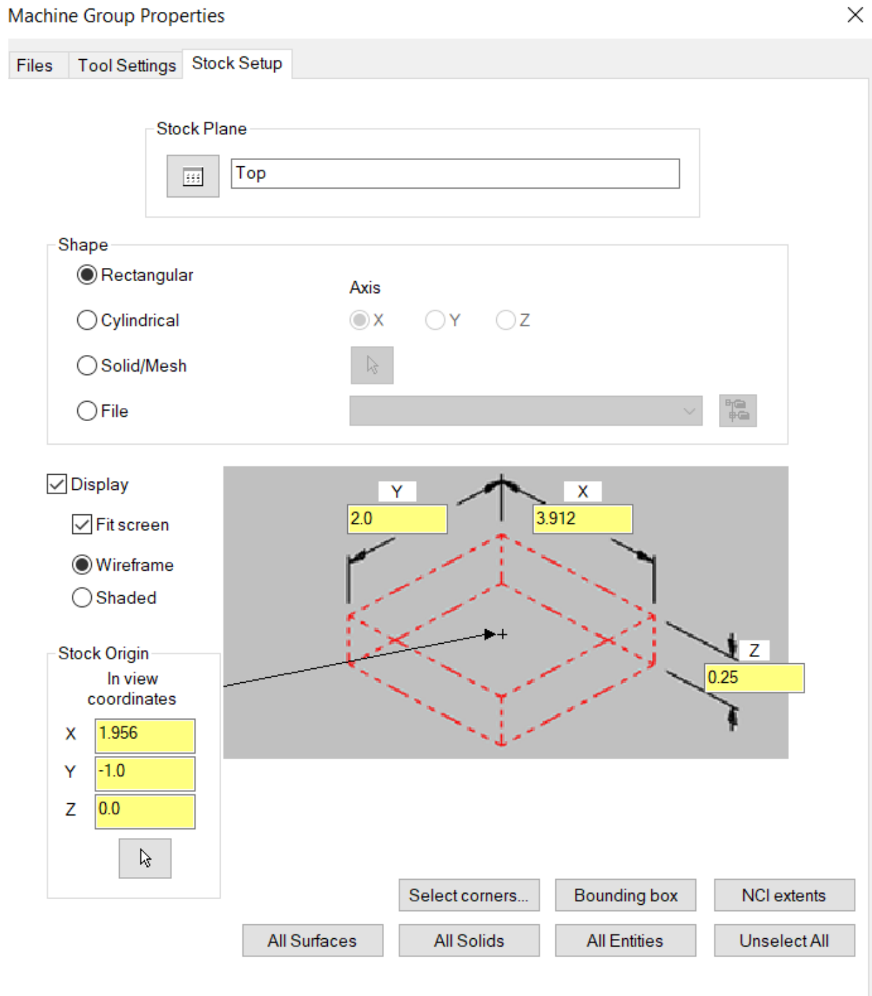
Figure 2 Stock Setting
