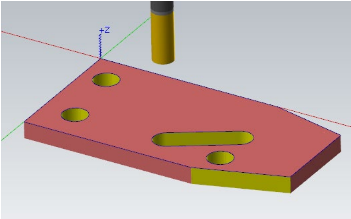
Figure 4 Verification of all operations
