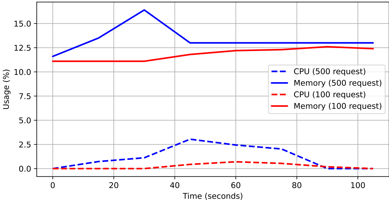
Statistics performance
