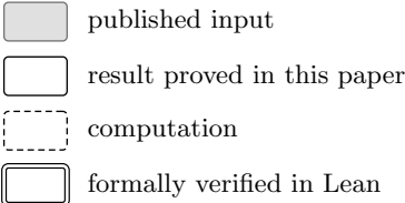
FIGURE 1. Proof map for Theorem 1.1 . An arrow points from a result to a result whose proof uses it; the joined lines into (R3) are the ingredients of Theorem 11.7 . The regimes (R1)–(R4) of Section 13 are defined by the first zero \lambda_1 , and (R2) splits at the constant u_{\text{exc}} of Section 12 . A double border marks a statement formally verified in Lean, with the published inputs as hypotheses, or, for the certificates, a computation accepted by a checker proved sound in Lean. The formalization also covers the far budget and parts of Propositions 9.7 and 11.6 ; the zero-location results, the case tree, the costs, the two-test row, the exterior regimes and the assembly are not formally verified ( Section 14.3 ). Some arrows are omitted, for instance from the explicit formulas to Sections 5 and 7 and into Theorem 12.6 .
