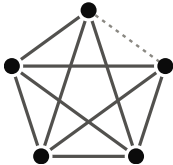
K_5 - e \rho = 3.2629
