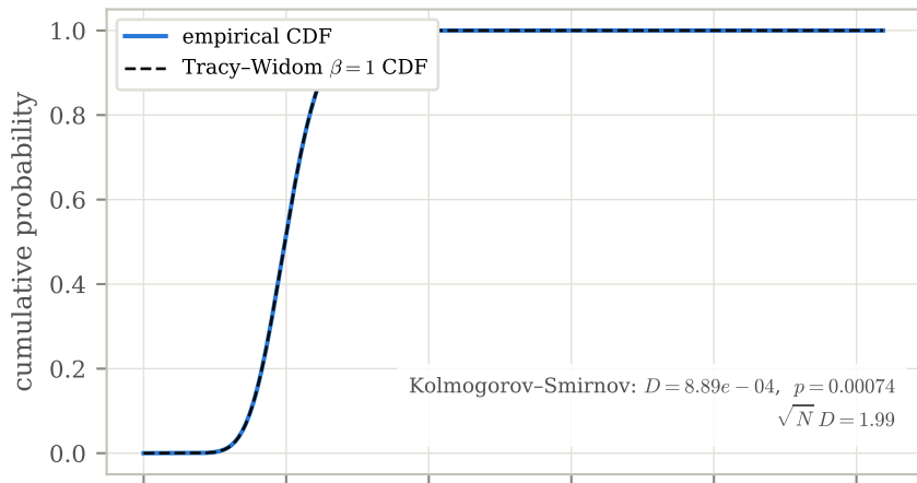
Empirical CDF vs Tracy-Widom \beta = 1 random covers of K_5 , V = 10,000 , N = 5,000,000
