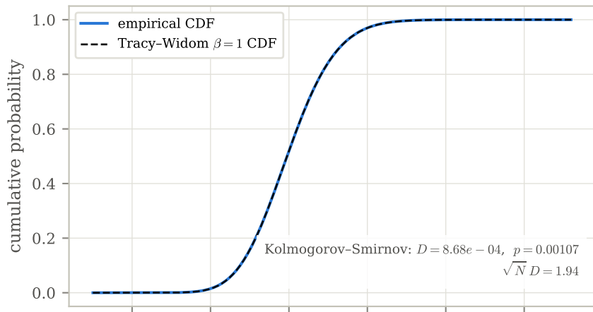
Empirical CDF vs Tracy-Widom \beta = 1 random simple 4-regular graphs, V = 20,000 , N = 5,000,000
