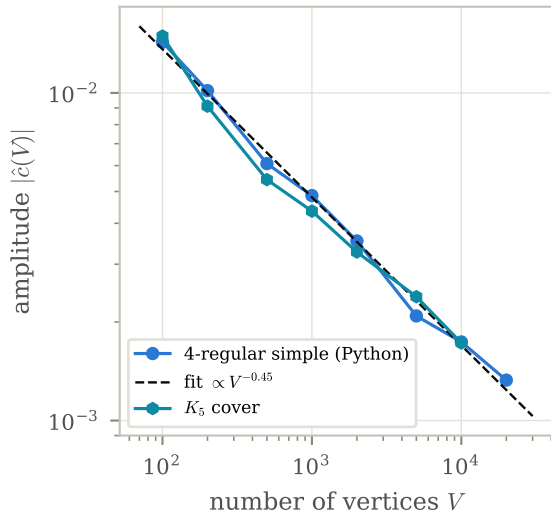
Edgeworth amplitude of the deviation
