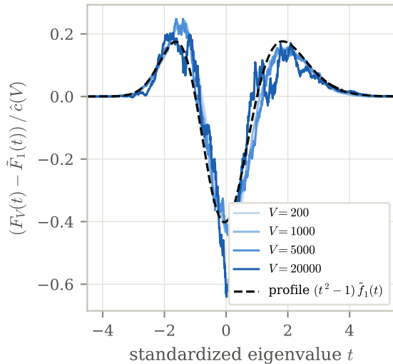
Rescaled deviations collapse
