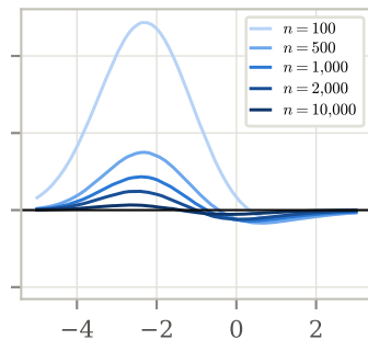
K_5 - e against TW_1 , predicted c_B
