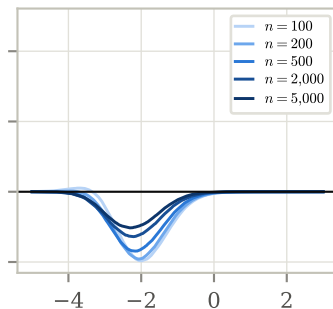
K_5 against TW_1
