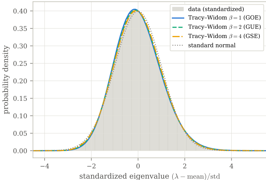
Density of \lambda vs Tracy-Widom laws random simple 4-regular graphs, V = 20,000 , N = 5,000,000
