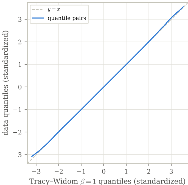
QQ plot vs Tracy-Widom \beta = 1 random simple 4-regular graphs, V = 500,000 , N = 100,000 (MATLAB)
