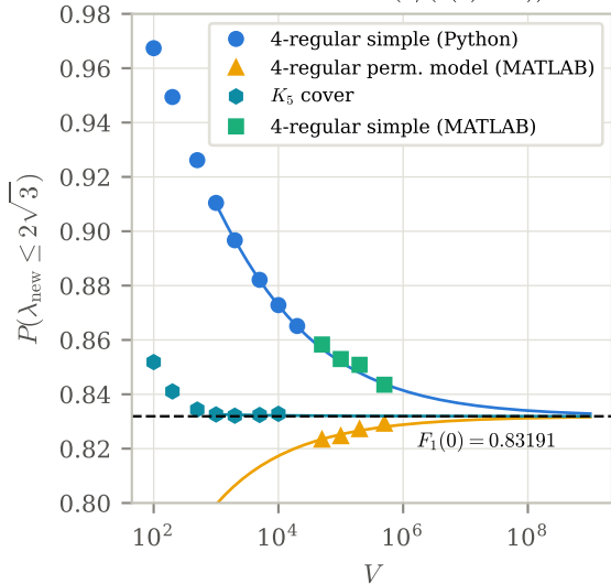
Data (markers) and F_1(a/(c(4)V^{1/3})) (lines)
