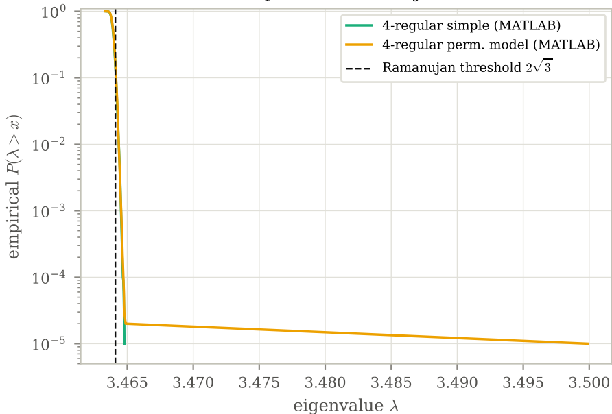
Right tail at V=500,000 : the multigraph model has far outliers past the Ramanujan threshold
