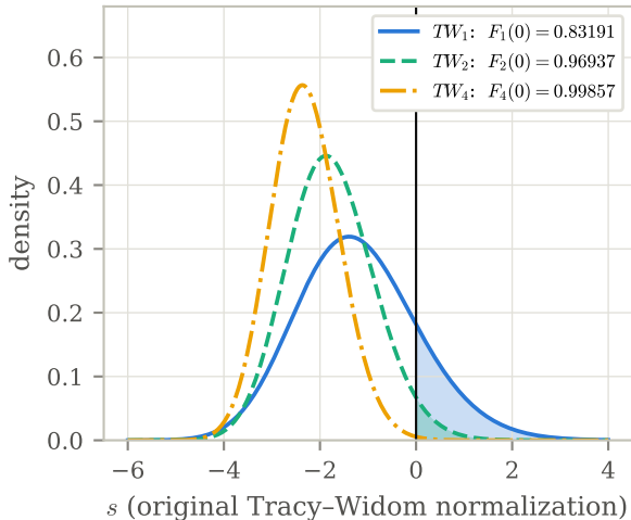
Pure laws (shaded: 1 - F_\beta(0) )
