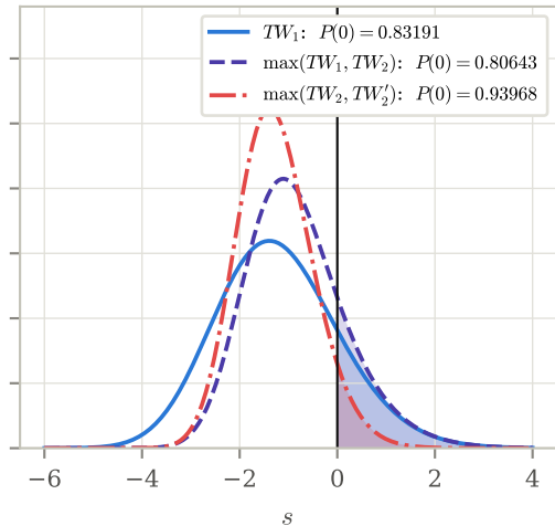
Maximum laws of the \mathbb{Z}_4 and \mathbb{Z}_5 covers
