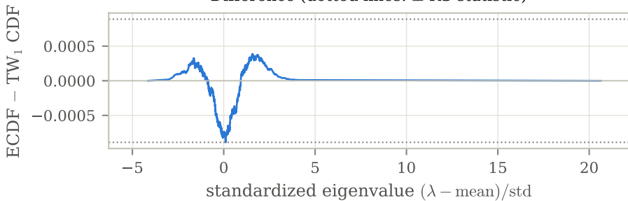
Difference (dotted lines: \pm KS statistic)
