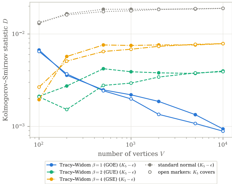
KS distance of standardized \lambda_{new} to candidate laws covers of K_5 - e (filled) and K_5 (open)
