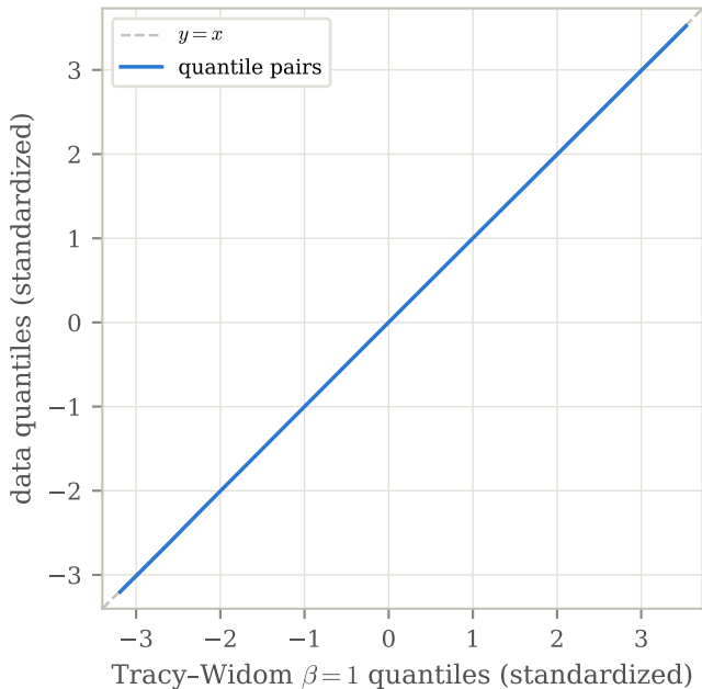
QQ plot vs Tracy-Widom \beta = 1 random covers of K_5 , V = 10,000 , N = 5,000,000
