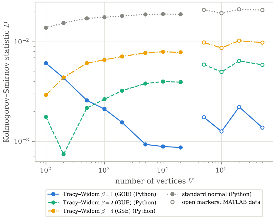
KS distance of standardized \lambda to candidate laws random simple 4-regular graphs
