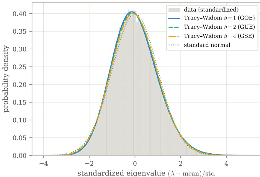
Density of \lambda vs Tracy-Widom laws random simple 4-regular graphs, V=500,000 , N=100,000 (MATLAB)
