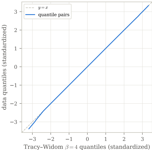
QQ plot vs Tracy-Widom \beta = 4 quaternion covers, V = 20,000 , N = 10^6
