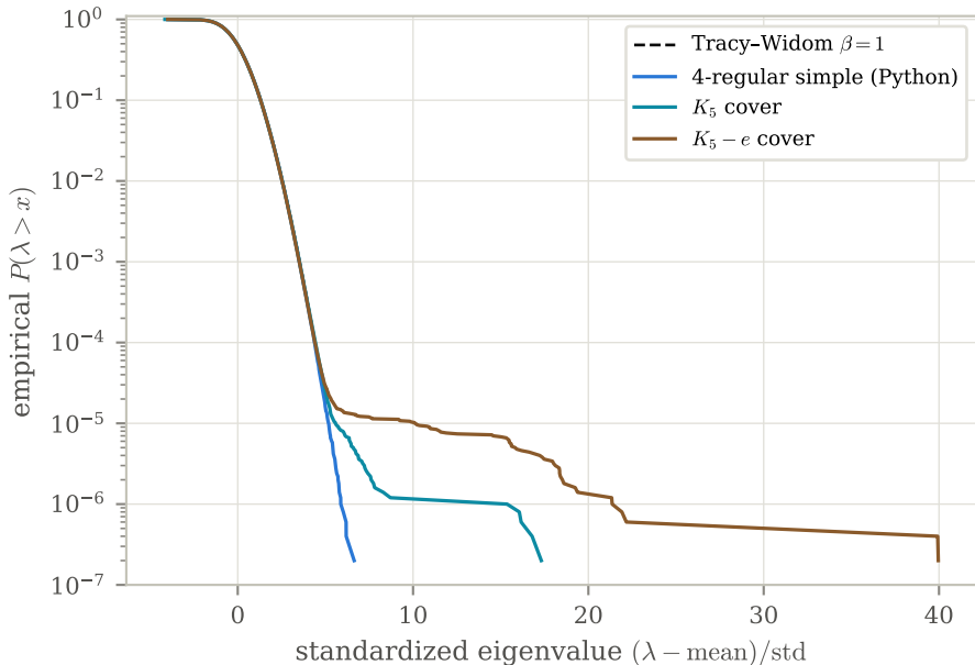
Standardized right tail at V=10,000 : thin far-outlier tails for the fixed-base cover families
